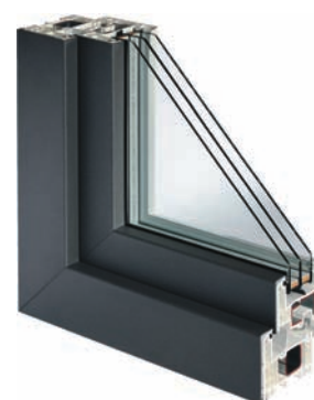
Kombisystem Alu 6 chamber system, construction depth: 83 mm. Aluminium cladding. Triple gasket system.
