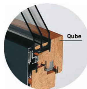
Alutrend Qube Two variants of internal finish: Standard (rounded), Qube (angular)
